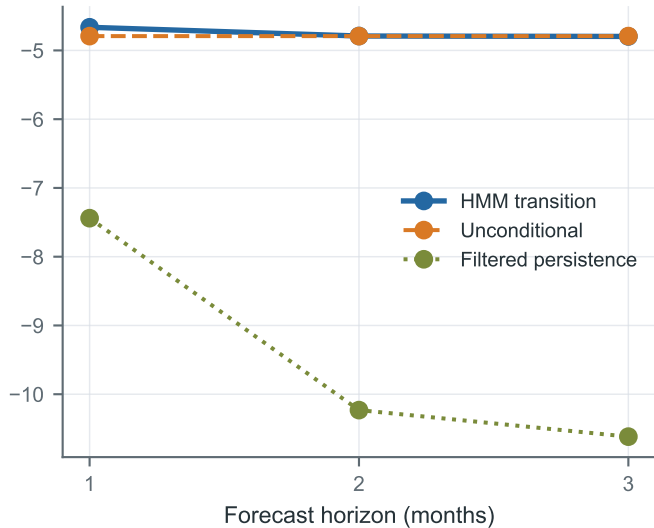
A. Held out predictive density
